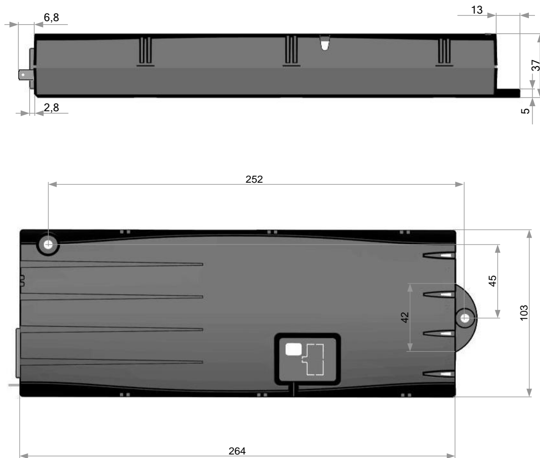
Figure 1: Dimensions in mm; Tolerances according to DIN ISO 2768-1 c
