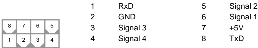
Figure 5: Pin assignment of LogicConnector DATA
