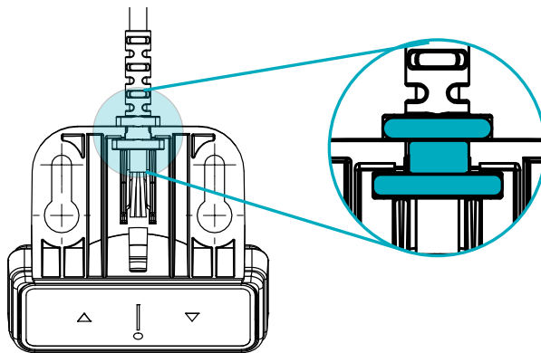
Fig. 9: Inserting the DMUI-TOUCH-B-UD Strain Relief
