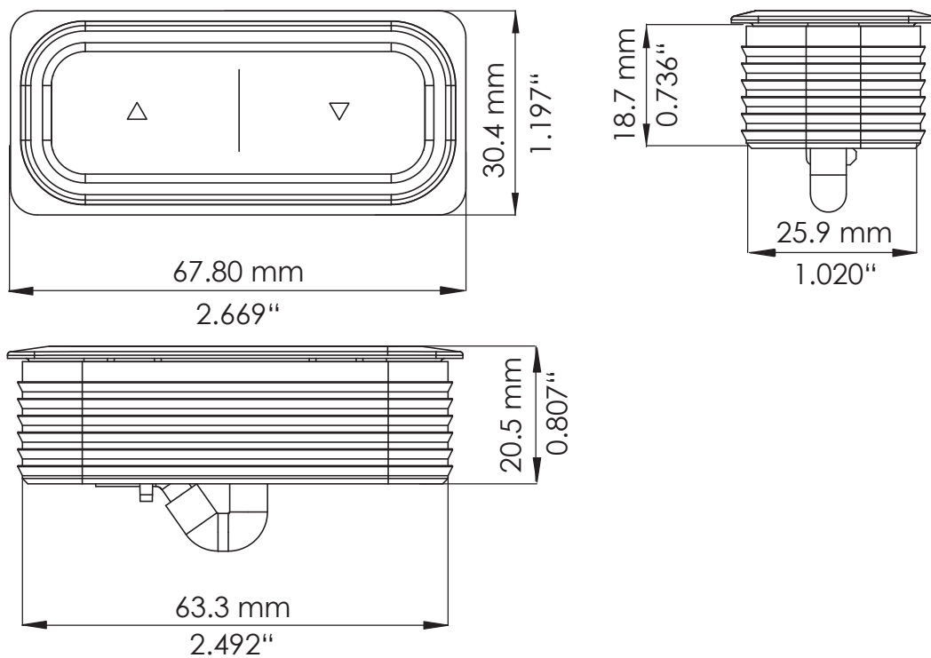
Fig. 5: Product dimensions, DMUI-TOUCH-B-IL
