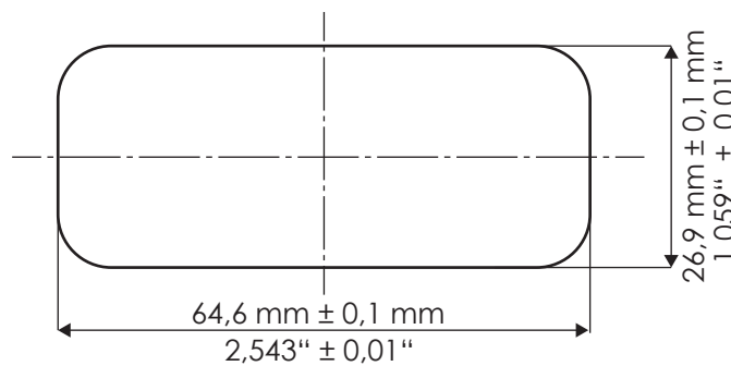
Fig. 6: Dimensions for the milled cut-out, DMUI-TOUCH-B-IL
