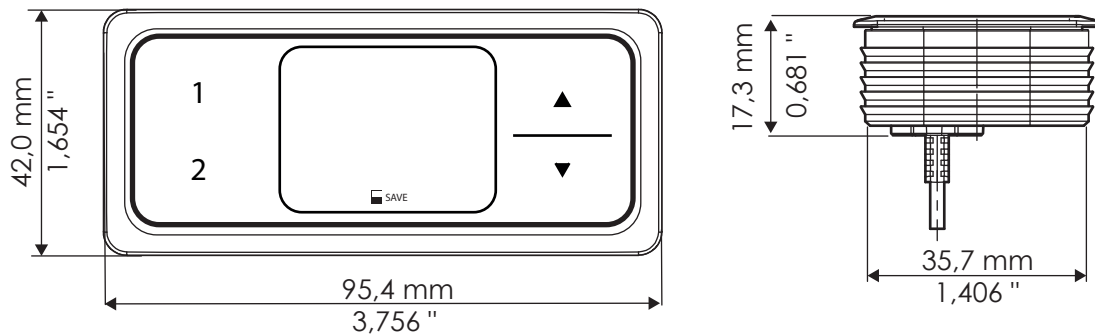
Fig. 3: Product dimensions, DMUI-TOUCH-C-IL
